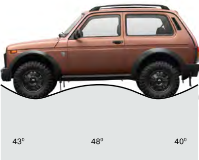
Approach angle, ramp angle, departure angle
